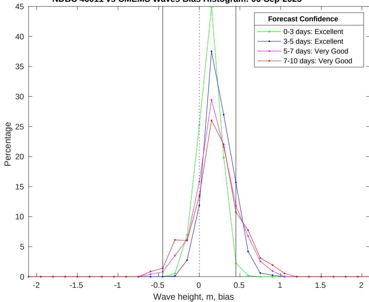
NDBC 46011 vs CMEMS Waves Bias Histogram: 06-Sep-2025
