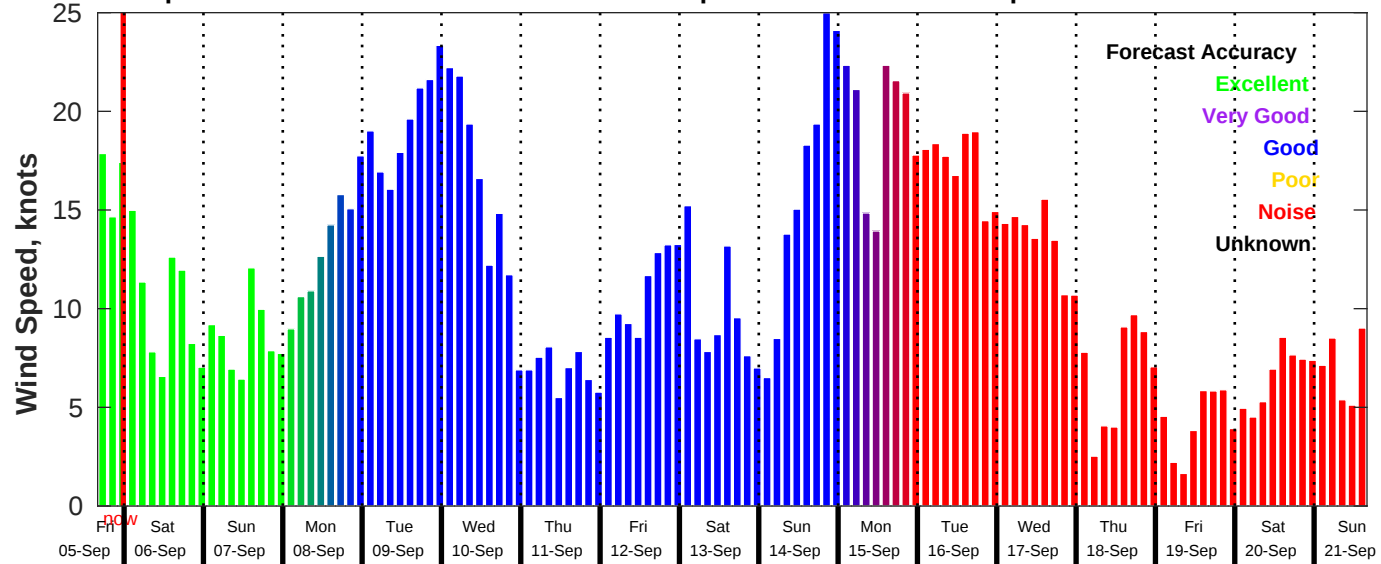
GFS Wind Speed Forecast for NDBC 46011 from 05-Sep-2025 16:00:00 to 21-Sep-2025 16:00:00
