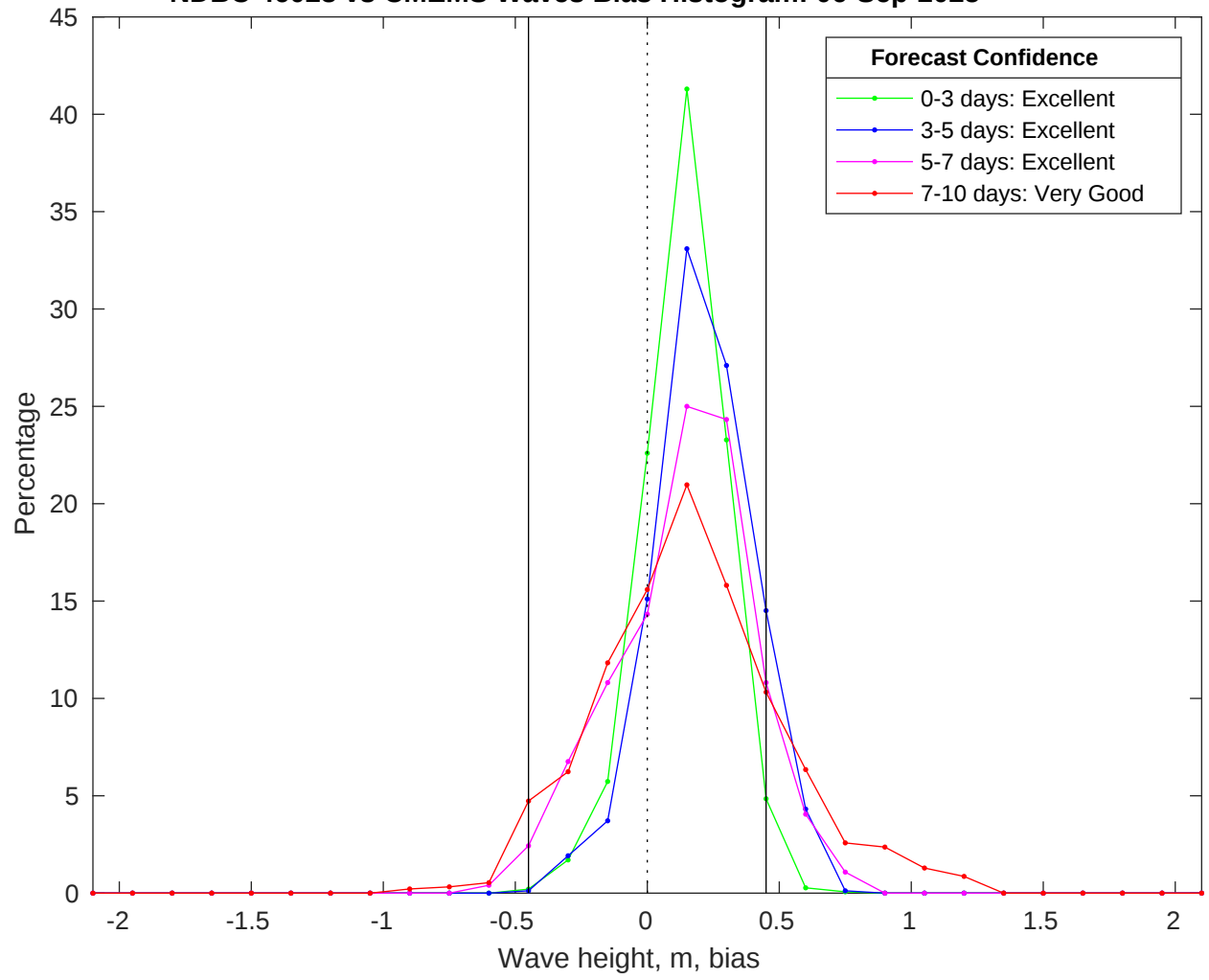
NDBC 46028 vs CMEMS Waves Bias Histogram: 06-Sep-2025
