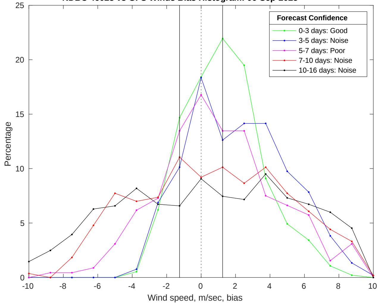
NDBC 46028 vs GFS Winds Bias Histogram: 06-Sep-2025
