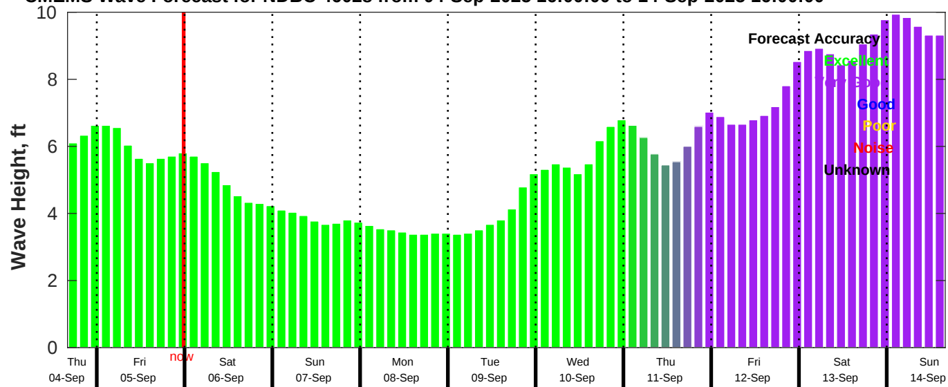
CMEMS Wave Forecast for NDBC 46028 from 04-Sep-2025 16:00:00 to 14-Sep-2025 16:00:00
