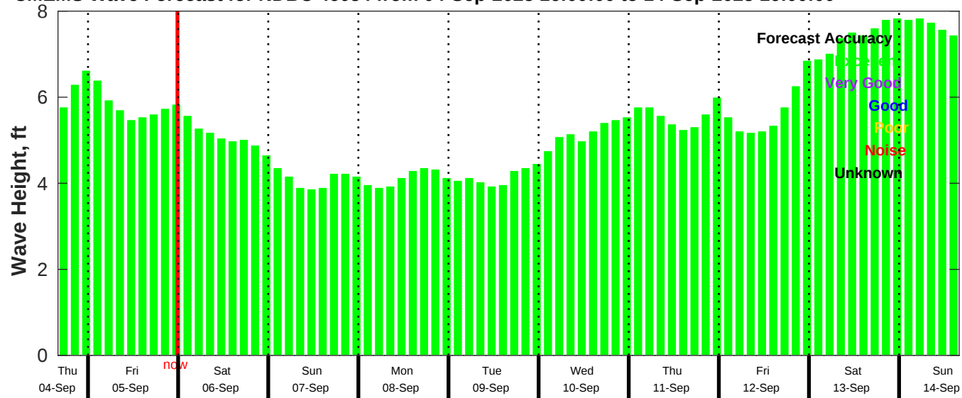
CMEMS Wave Forecast for NDBC 46054 from 04-Sep-2025 16:00:00 to 14-Sep-2025 16:00:00
