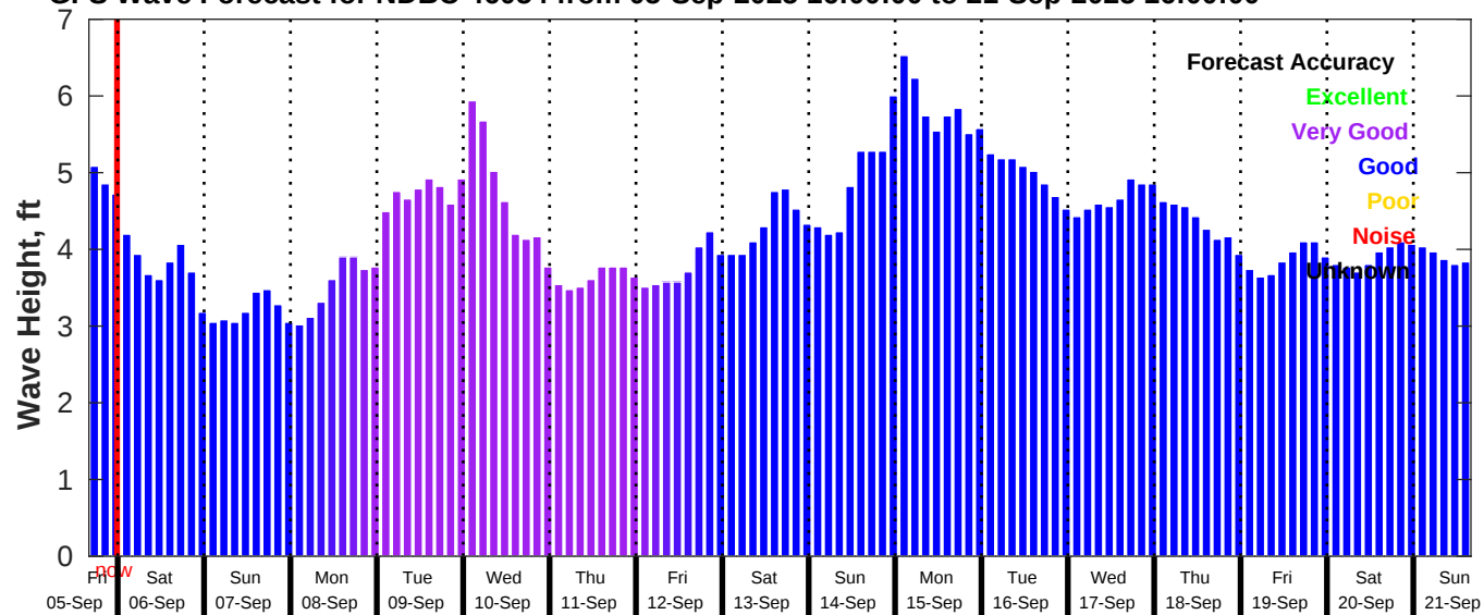
GFS Wave Forecast for NDBC 46054 from 05-Sep-2025 16:00:00 to 21-Sep-2025 16:00:00
