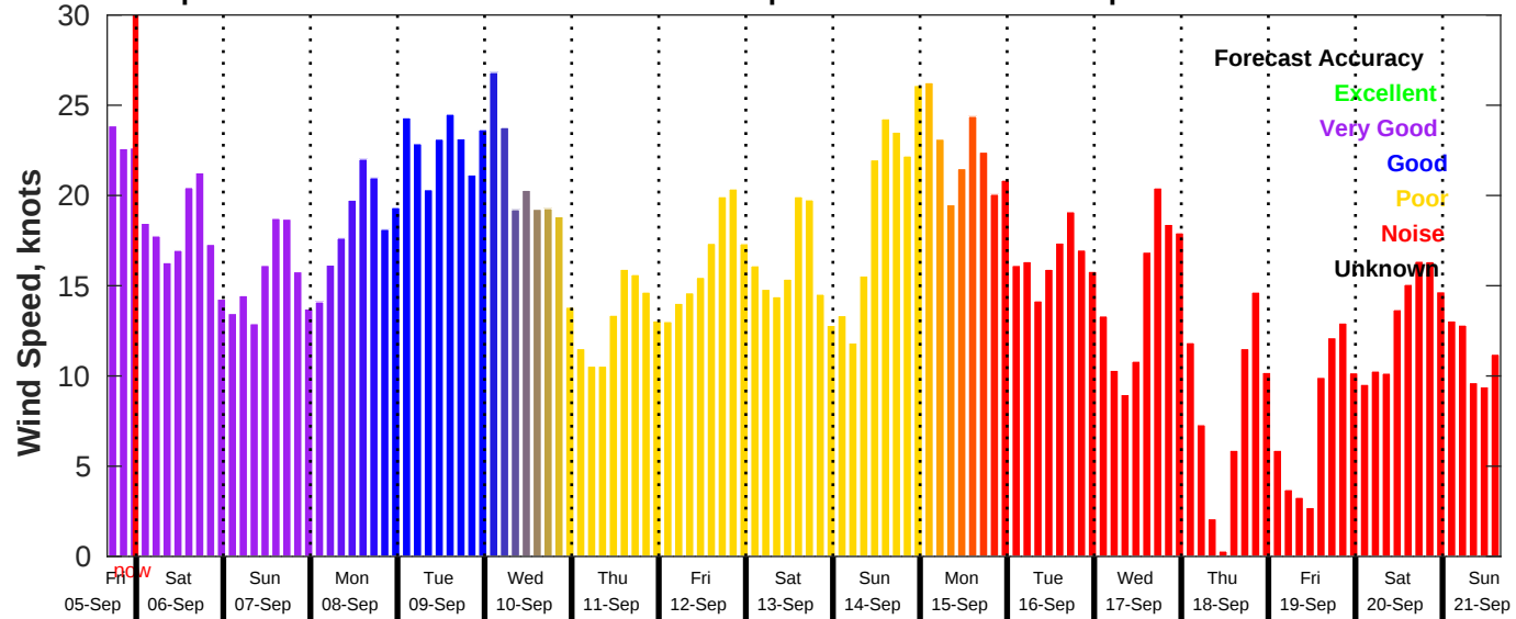
GFS Wind Speed Forecast for NDBC 46054 from 05-Sep-2025 16:00:00 to 21-Sep-2025 16:00:00
