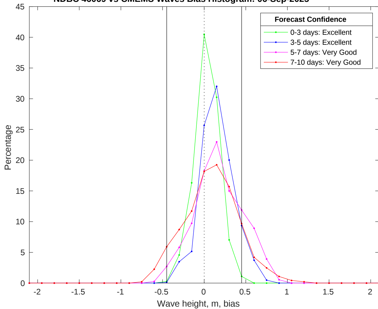
NDBC 46069 vs CMEMS Waves Bias Histogram: 06-Sep-2025
