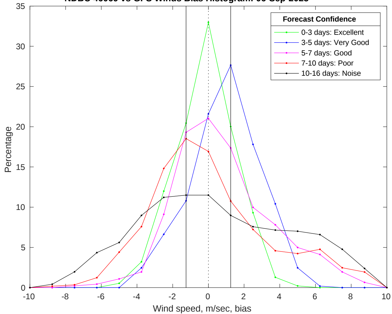
NDBC 46069 vs GFS Winds Bias Histogram: 06-Sep-2025
