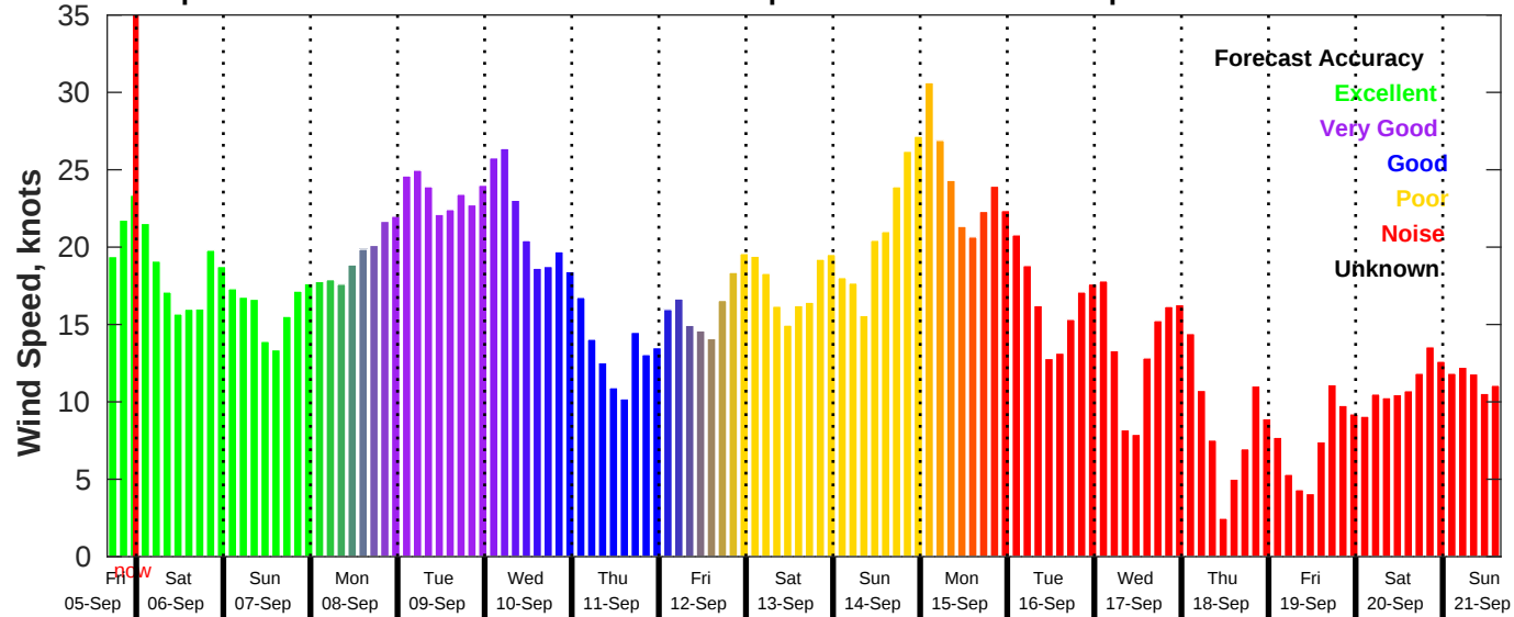
GFS Wind Speed Forecast for NDBC 46069 from 05-Sep-2025 16:00:00 to 21-Sep-2025 16:00:00
