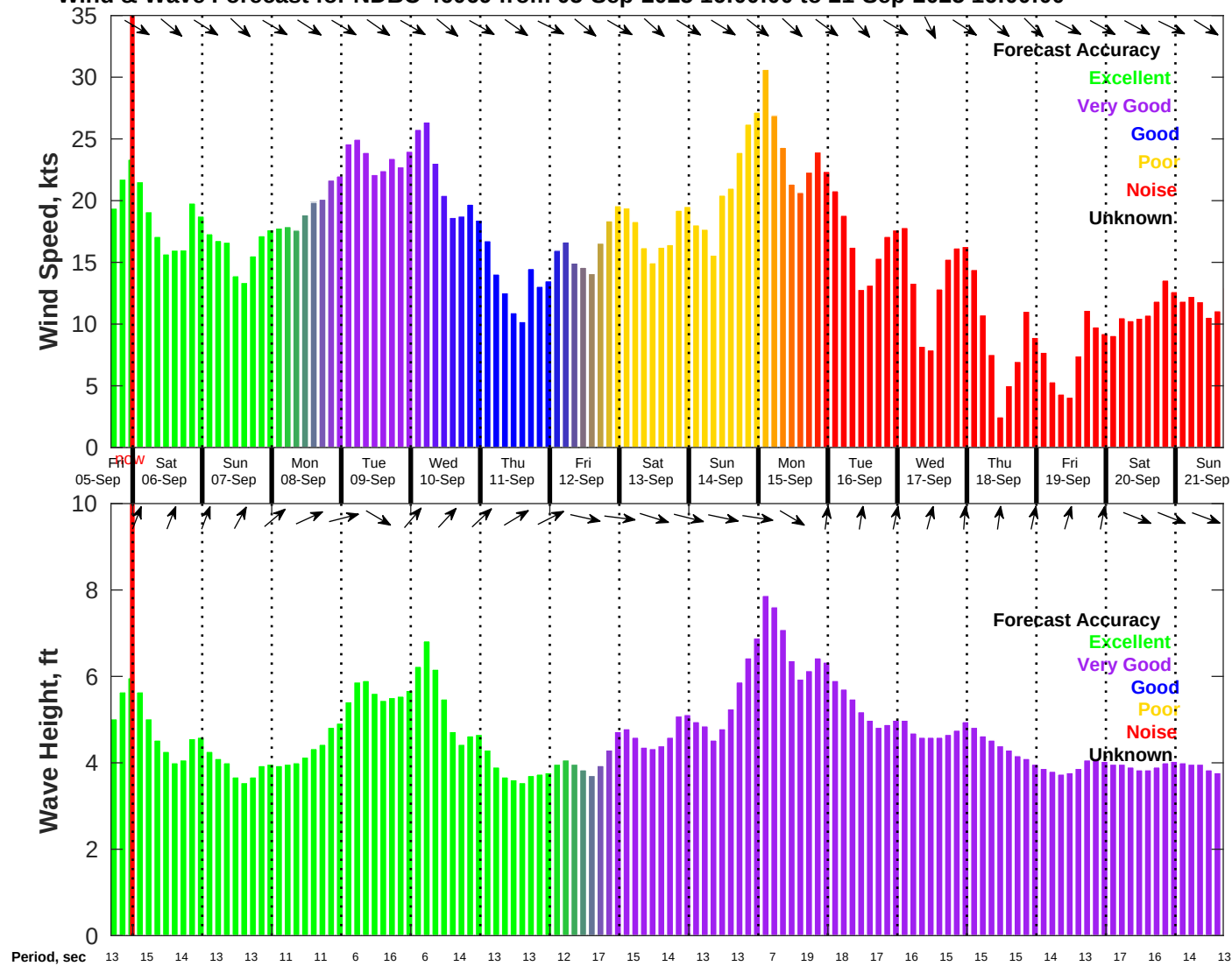
Wind & Wave Forecast for NDBC 46069 from 05-Sep-2025 16:00:00 to 21-Sep-2025 16:00:00
