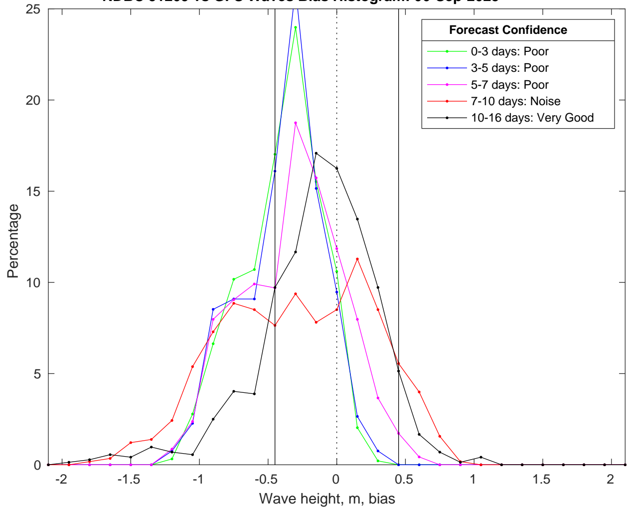
NDBC 51209 vs GFS Waves Bias Histogram: 06-Sep-2025
