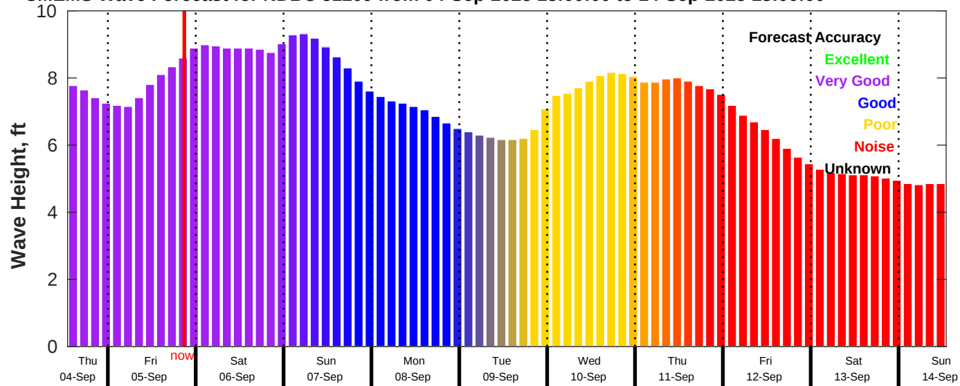
CMEMS Wave Forecast for NDBC 51209 from 04-Sep-2025 13:00:00 to 14-Sep-2025 13:00:00
