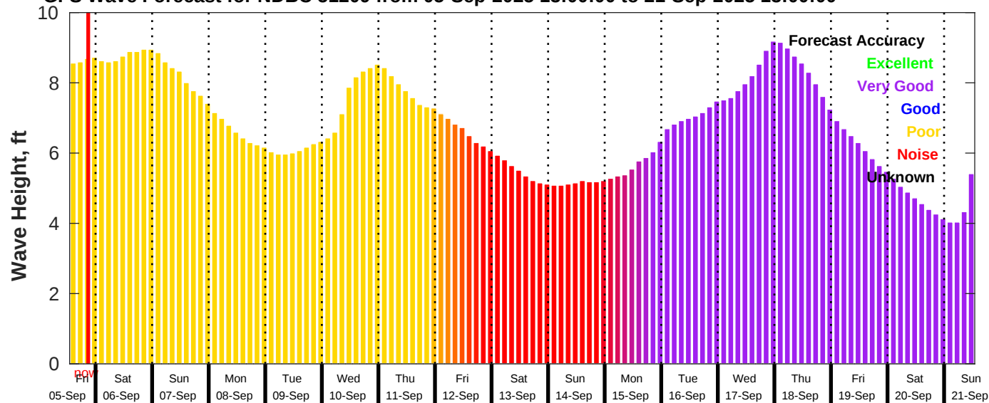
GFS Wave Forecast for NDBC 51209 from 05-Sep-2025 13:00:00 to 21-Sep-2025 13:00:00
