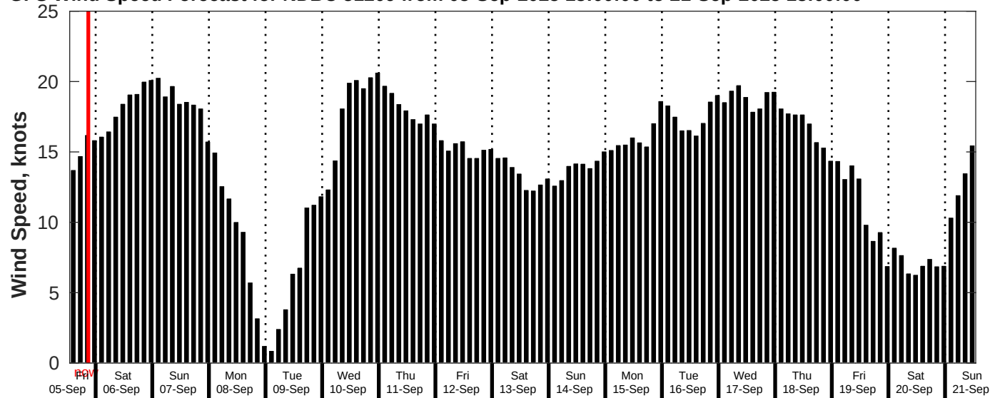
GFS Wind Speed Forecast for NDBC 51209 from 05-Sep-2025 13:00:00 to 21-Sep-2025 13:00:00
