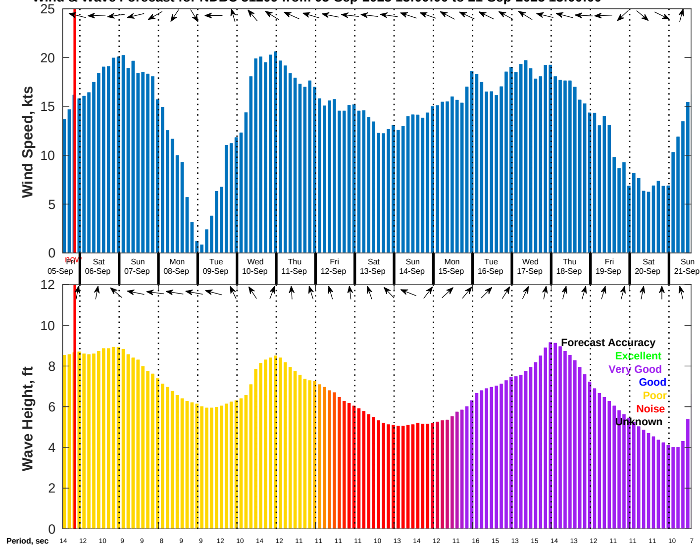
Wind & Wave Forecast for NDBC 51209 from 05-Sep-2025 13:00:00 to 21-Sep-2025 13:00:00
