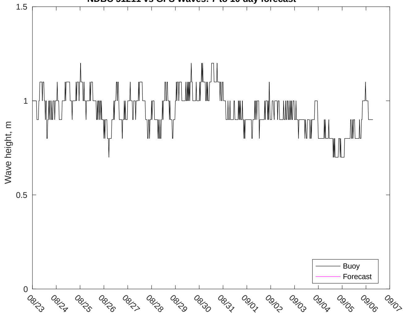
NDBC 51211 vs GFS Waves: 7 to 10 day forecast
