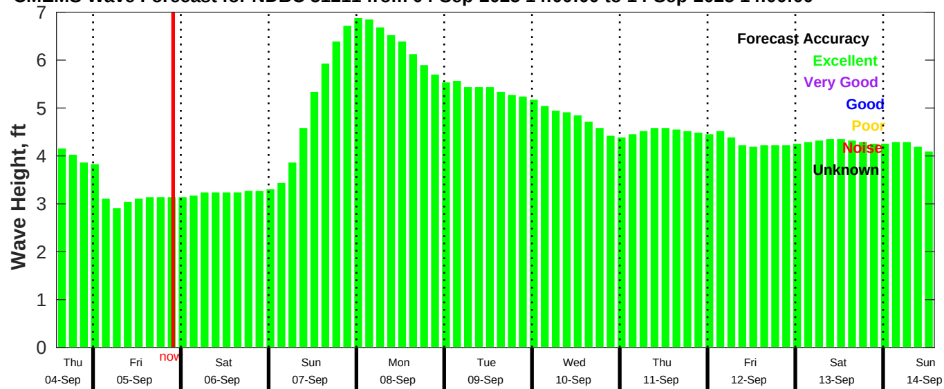
CMEMS Wave Forecast for NDBC 51211 from 04-Sep-2025 14:00:00 to 14-Sep-2025 14:00:00
