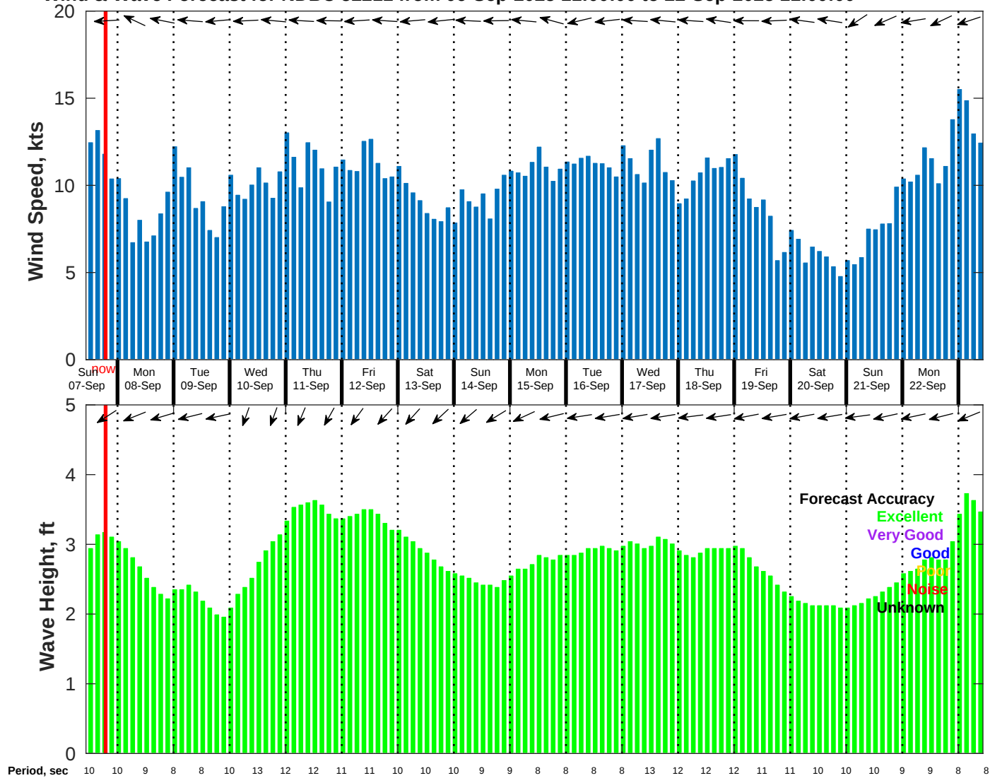
Wind & Wave Forecast for NDBC 52211 from 06-Sep-2025 11:00:00 to 22-Sep-2025 11:00:00
