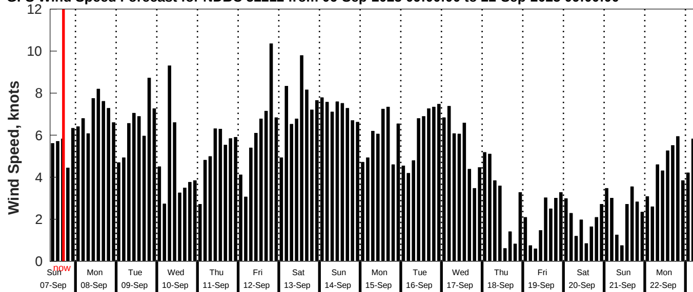
GFS Wind Speed Forecast for NDBC 52212 from 06-Sep-2025 09:00:00 to 22-Sep-2025 09:00:00
