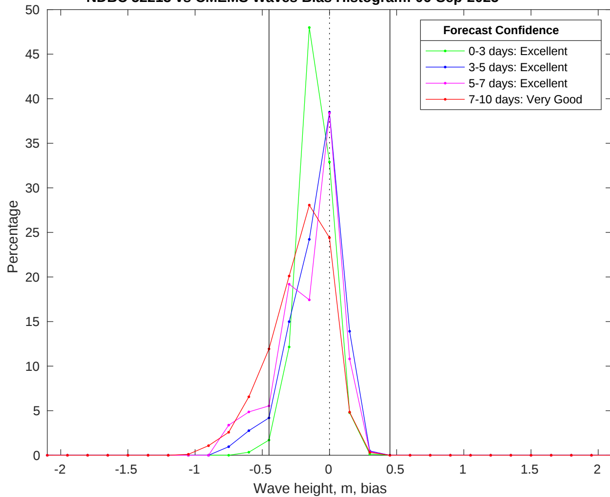
NDBC 52213 vs CMEMS Waves Bias Histogram: 06-Sep-2025
