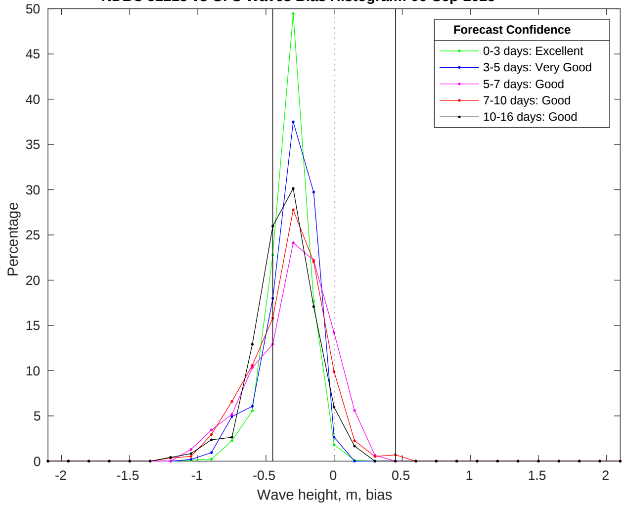
NDBC 52213 vs GFS Waves Bias Histogram: 06-Sep-2025
