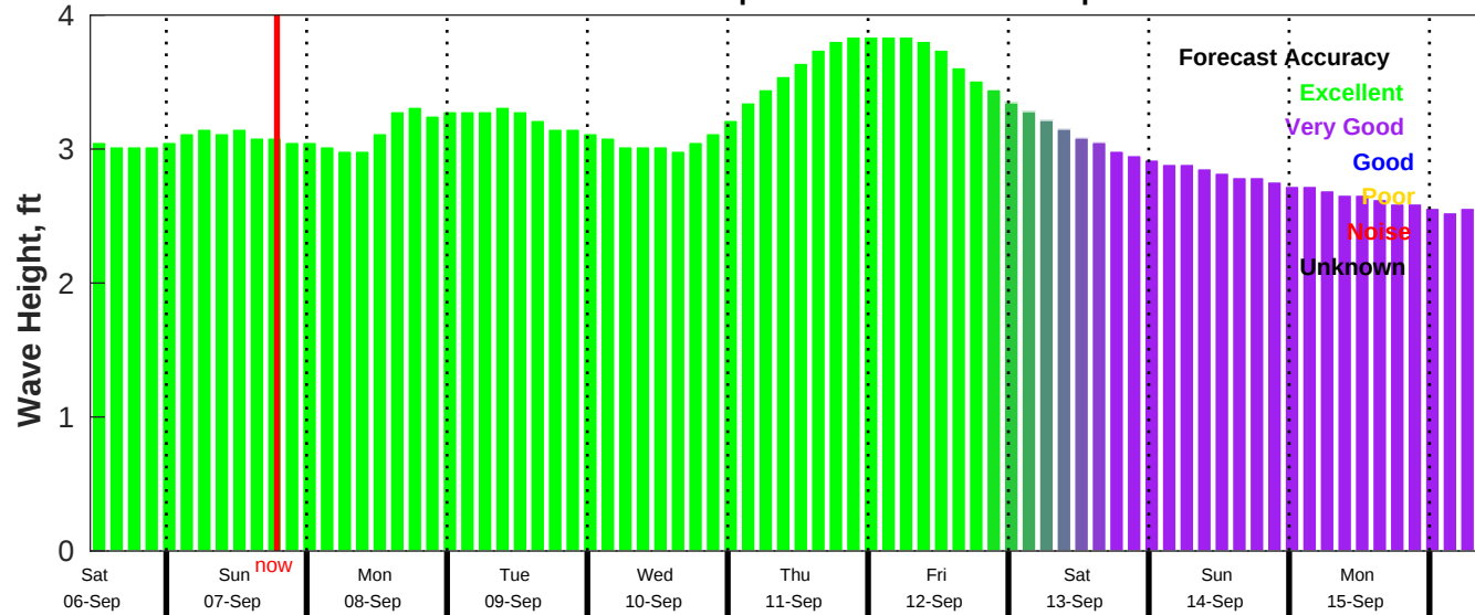
CMEMS Wave Forecast for NDBC 52213 from 05-Sep-2025 11:00:00 to 15-Sep-2025 11:00:00
