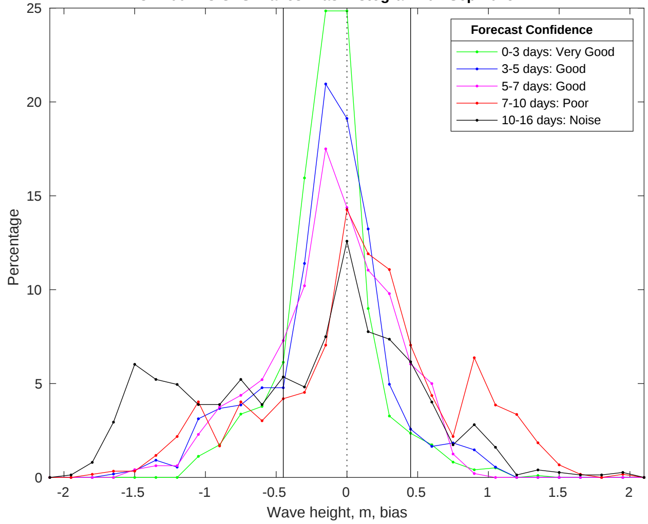
NDBC 41004 vs GFS Waves Bias Histogram: 07-Sep-2025
