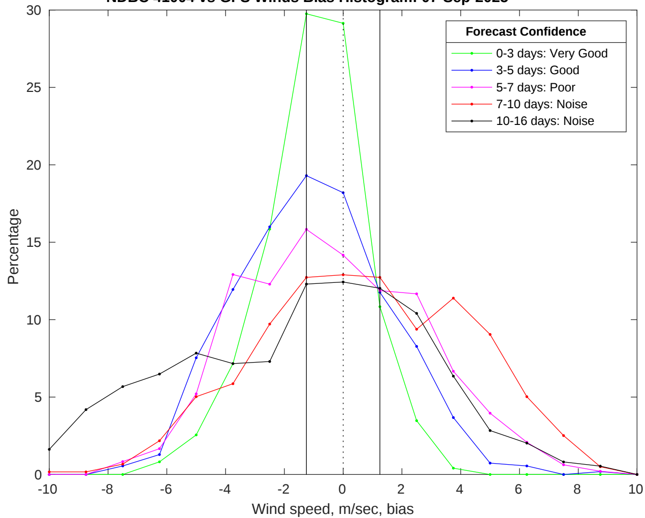
NDBC 41004 vs GFS Winds Bias Histogram: 07-Sep-2025
