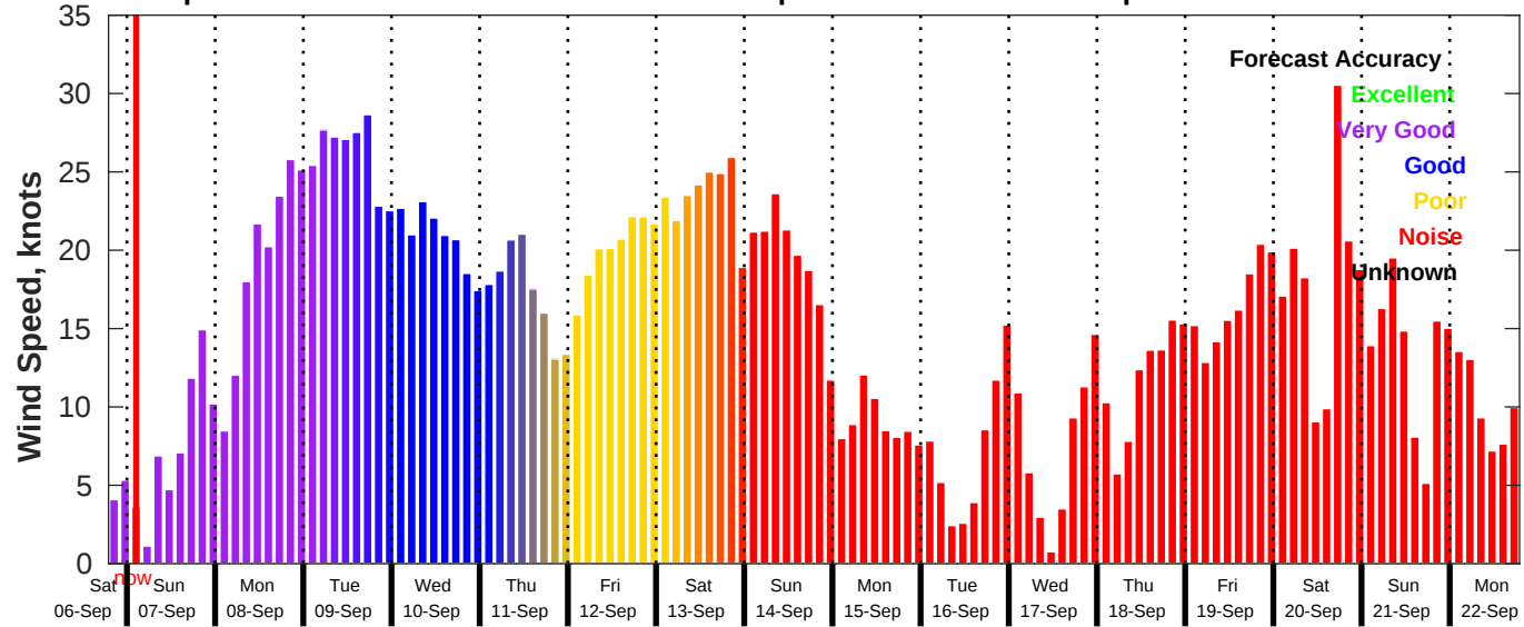
GFS Wind Speed Forecast for NDBC 41004 from 06-Sep-2025 19:00:00 to 22-Sep-2025 19:00:00
