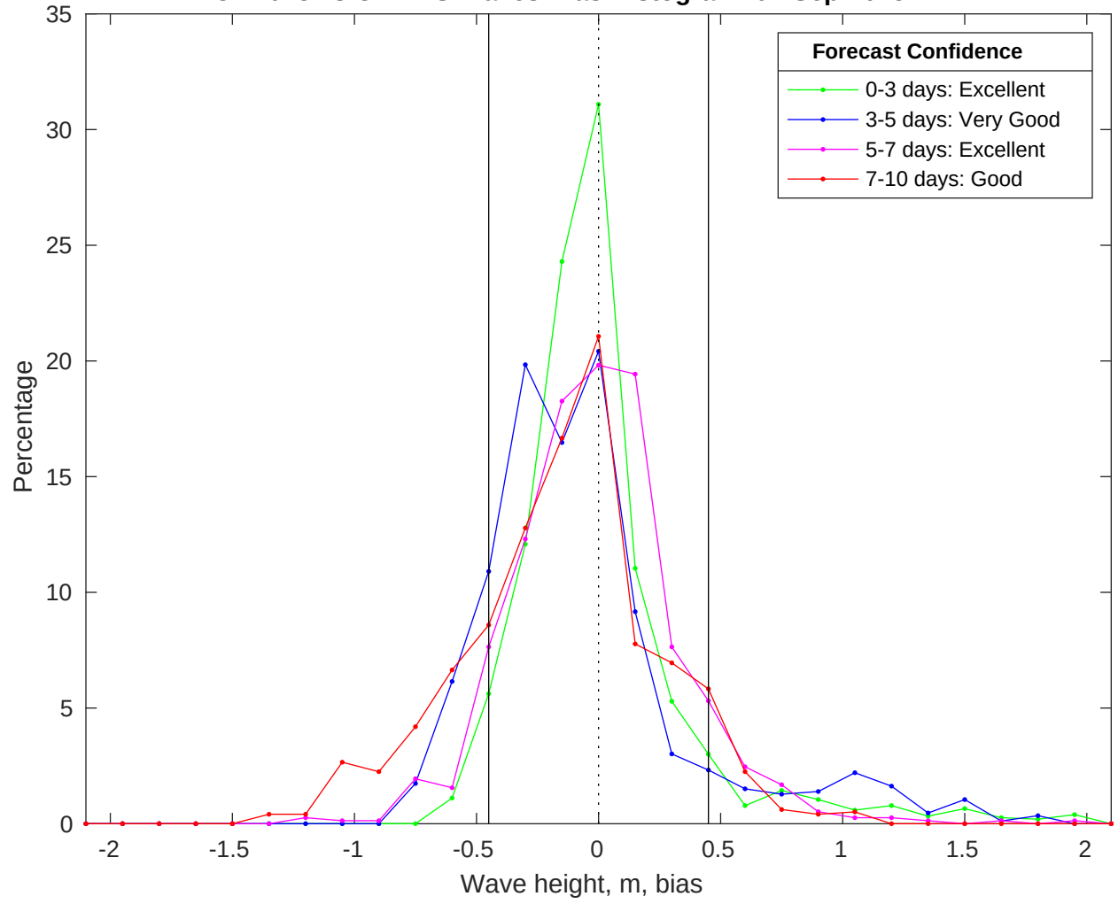
NDBC 41013 vs CMEMS Waves Bias Histogram: 07-Sep-2025
