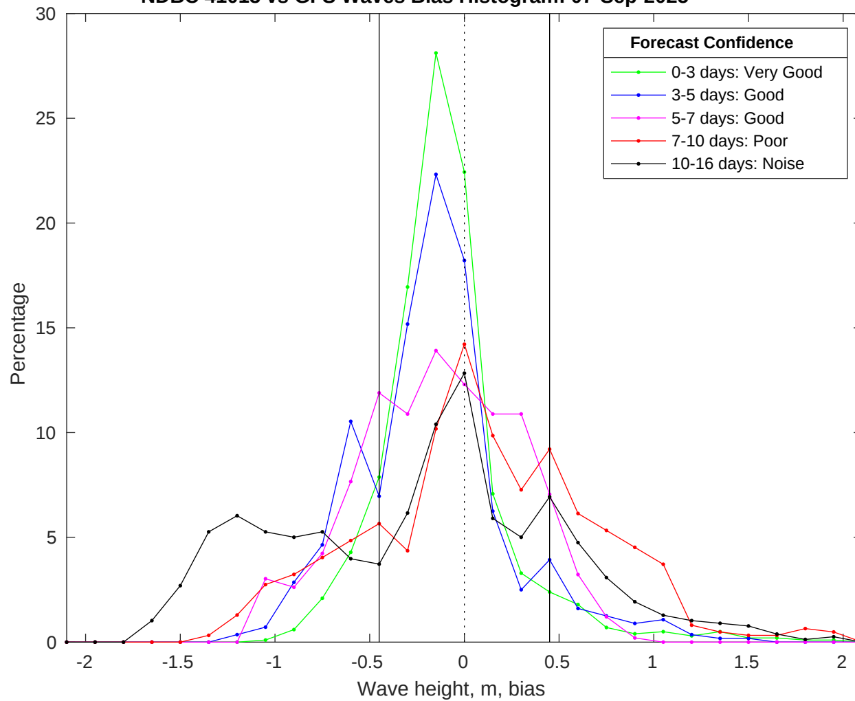
NDBC 41013 vs GFS Waves Bias Histogram: 07-Sep-2025
