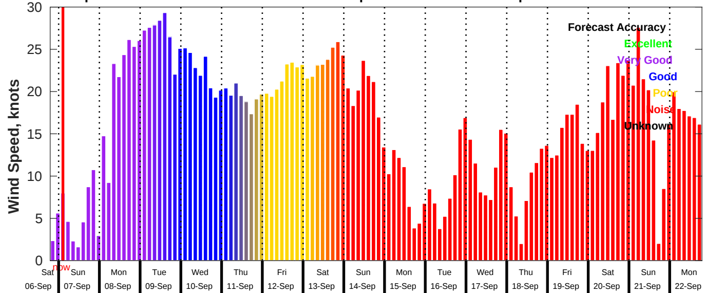
GFS Wind Speed Forecast for NDBC 41013 from 06-Sep-2025 19:00:00 to 22-Sep-2025 19:00:00
