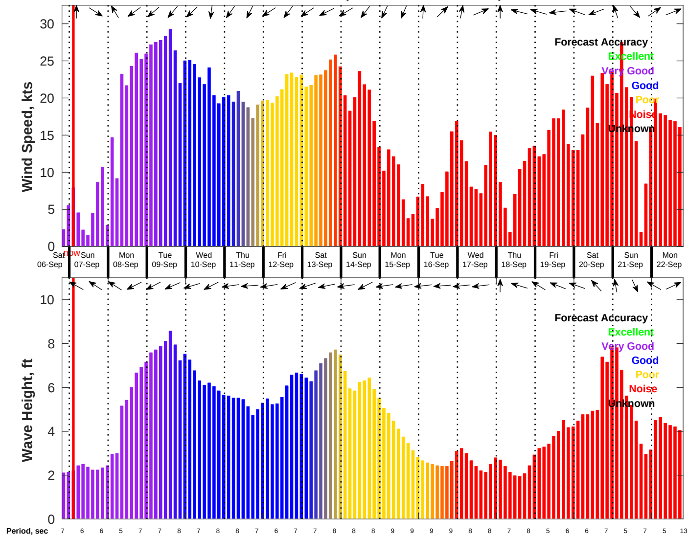
Wind & Wave Forecast for NDBC 41013 from 06-Sep-2025 19:00:00 to 22-Sep-2025 19:00:00
