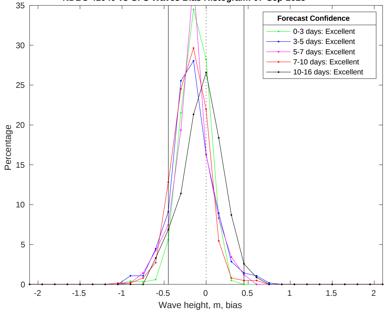
NDBC 41040 vs GFS Waves Bias Histogram: 07-Sep-2025
