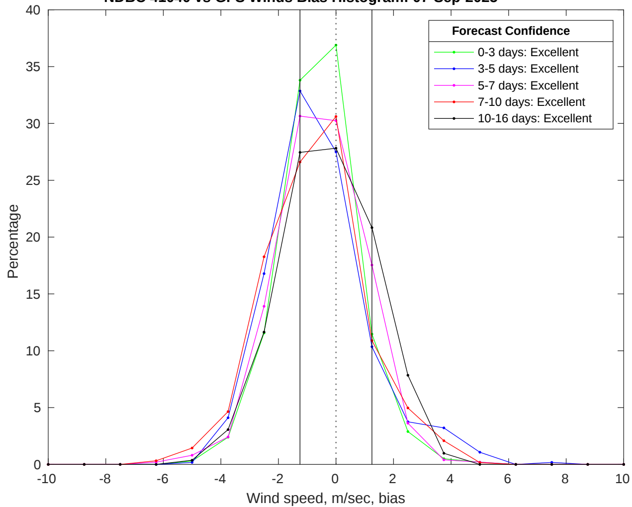
NDBC 41040 vs GFS Winds Bias Histogram: 07-Sep-2025
