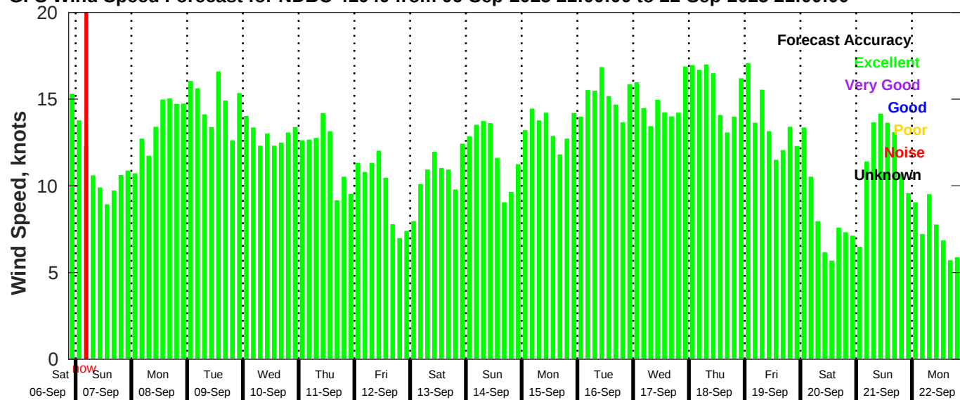
GFS Wind Speed Forecast for NDBC 41040 from 06-Sep-2025 21:00:00 to 22-Sep-2025 21:00:00
