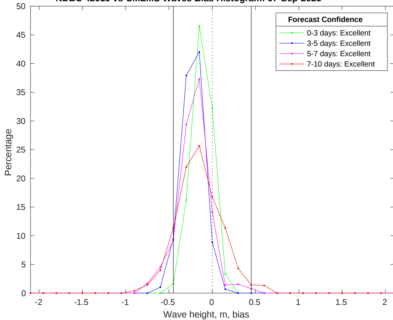
NDBC 42019 vs CMEMS Waves Bias Histogram: 07-Sep-2025
