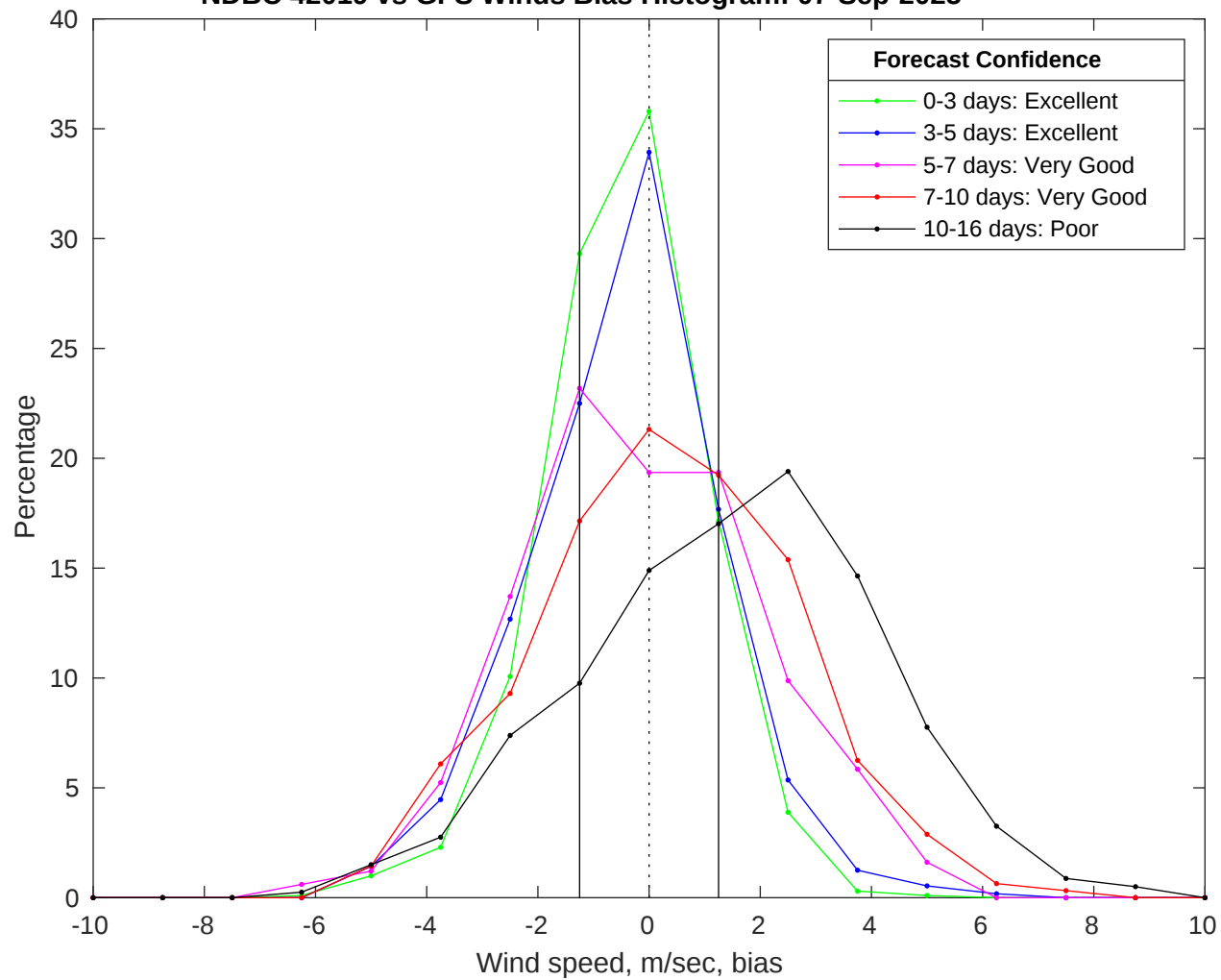
NDBC 42019 vs GFS Winds Bias Histogram: 07-Sep-2025
