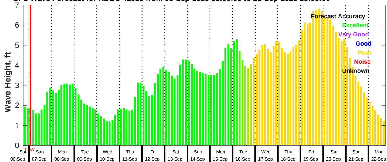
GFS Wave Forecast for NDBC 42019 from 06-Sep-2025 18:00:00 to 22-Sep-2025 18:00:00
