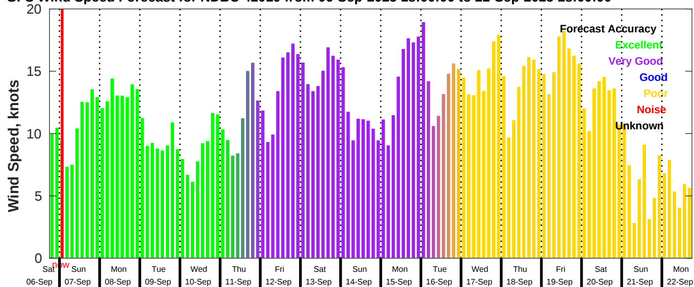
GFS Wind Speed Forecast for NDBC 42019 from 06-Sep-2025 18:00:00 to 22-Sep-2025 18:00:00
