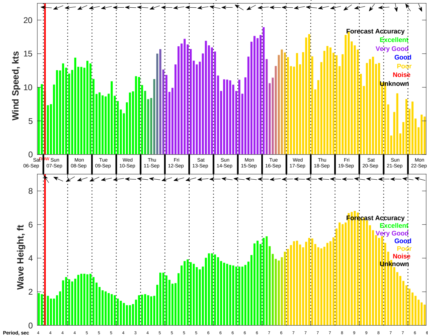
Wind & Wave Forecast for NDBC 42019 from 06-Sep-2025 18:00:00 to 22-Sep-2025 18:00:00
