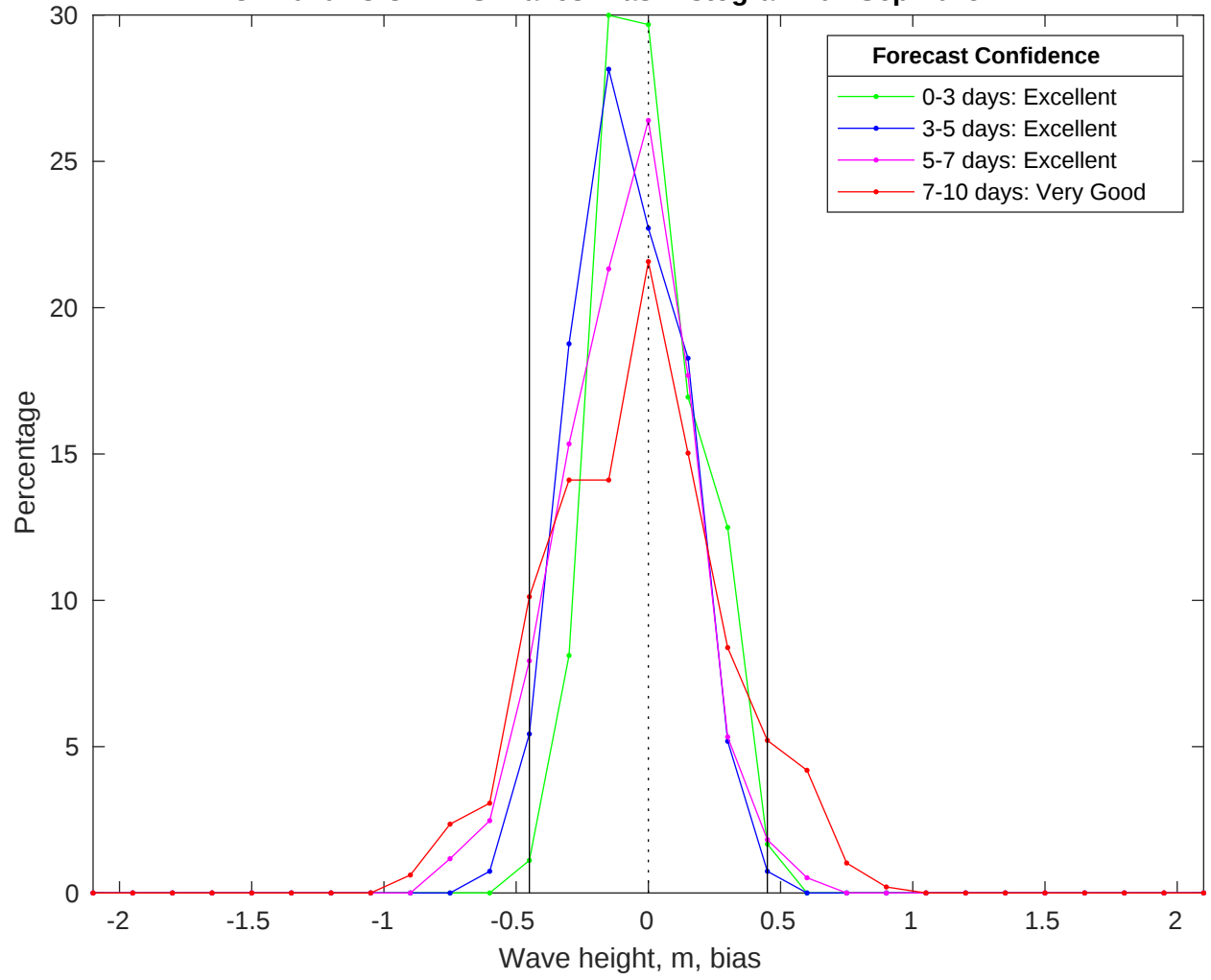
NDBC 42020 vs CMEMS Waves Bias Histogram: 07-Sep-2025
