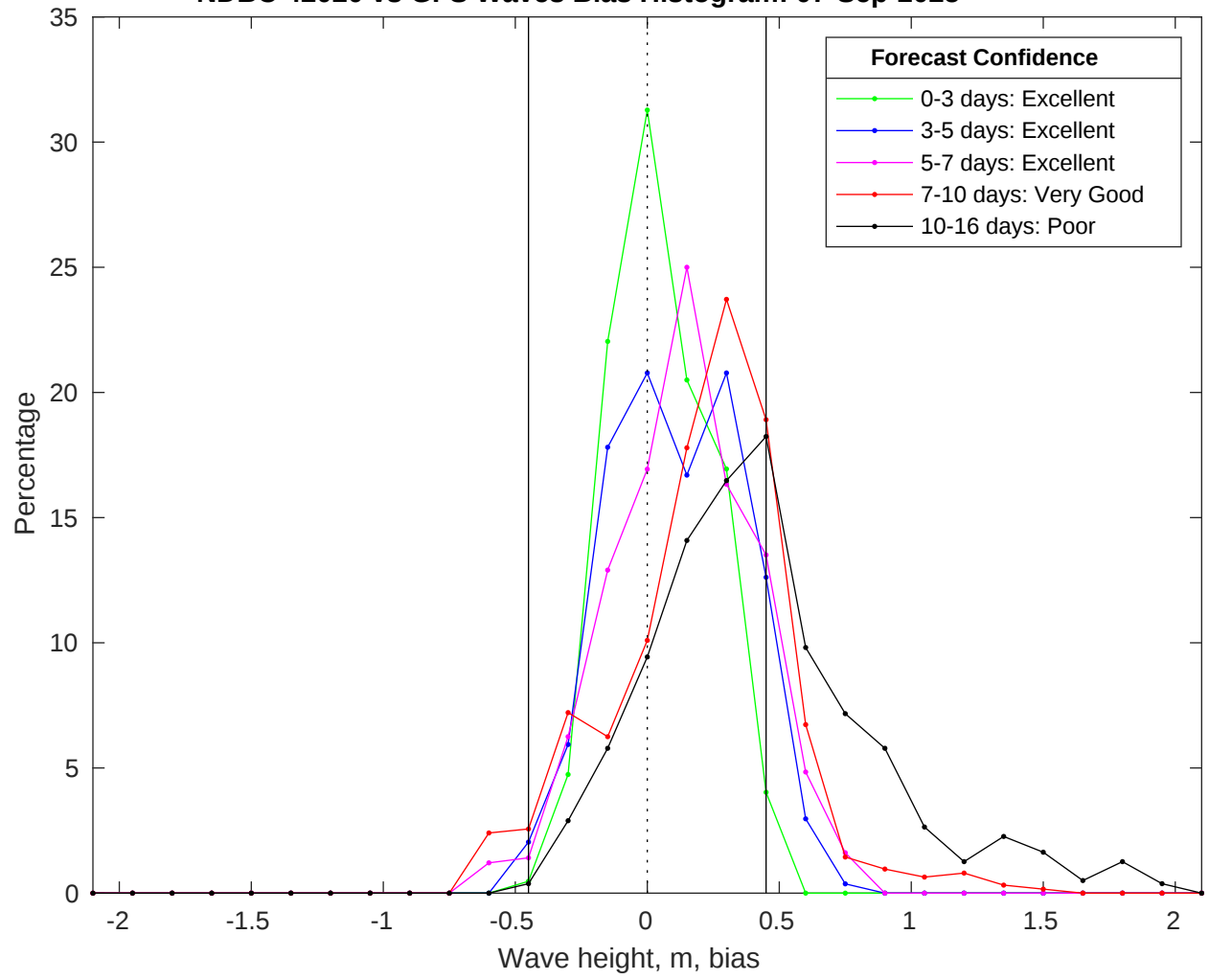
NDBC 42020 vs GFS Waves Bias Histogram: 07-Sep-2025
