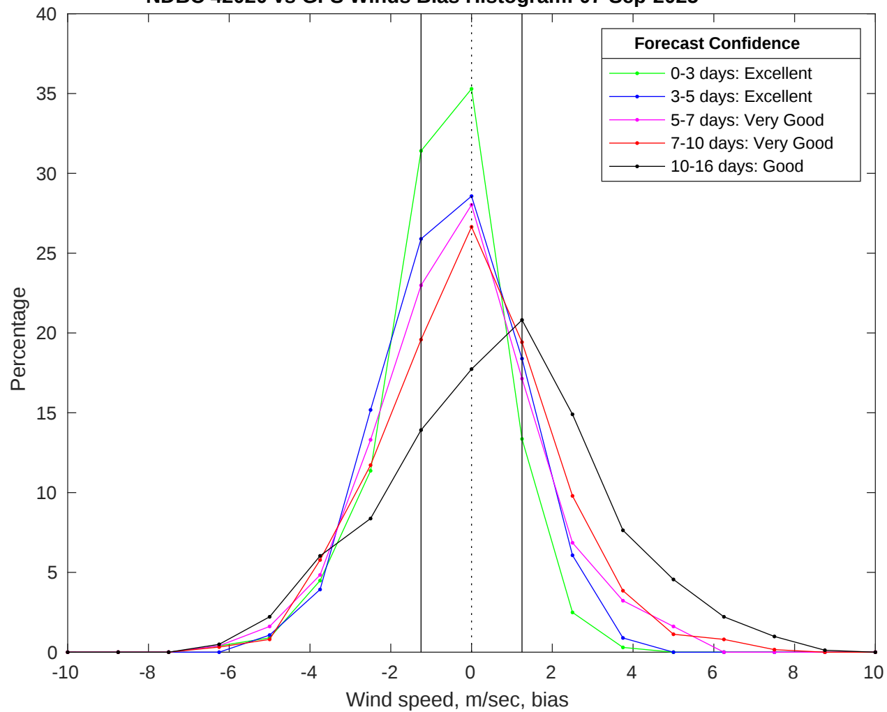
NDBC 42020 vs GFS Winds Bias Histogram: 07-Sep-2025
