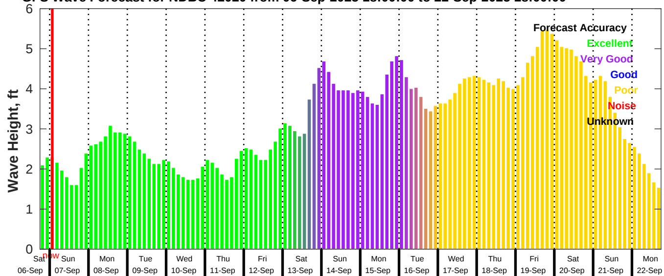
GFS Wave Forecast for NDBC 42020 from 06-Sep-2025 18:00:00 to 22-Sep-2025 18:00:00
