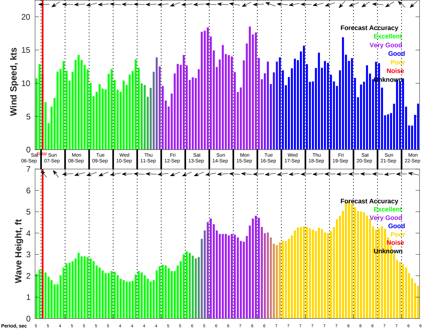
Wind & Wave Forecast for NDBC 42020 from 06-Sep-2025 18:00:00 to 22-Sep-2025 18:00:00
