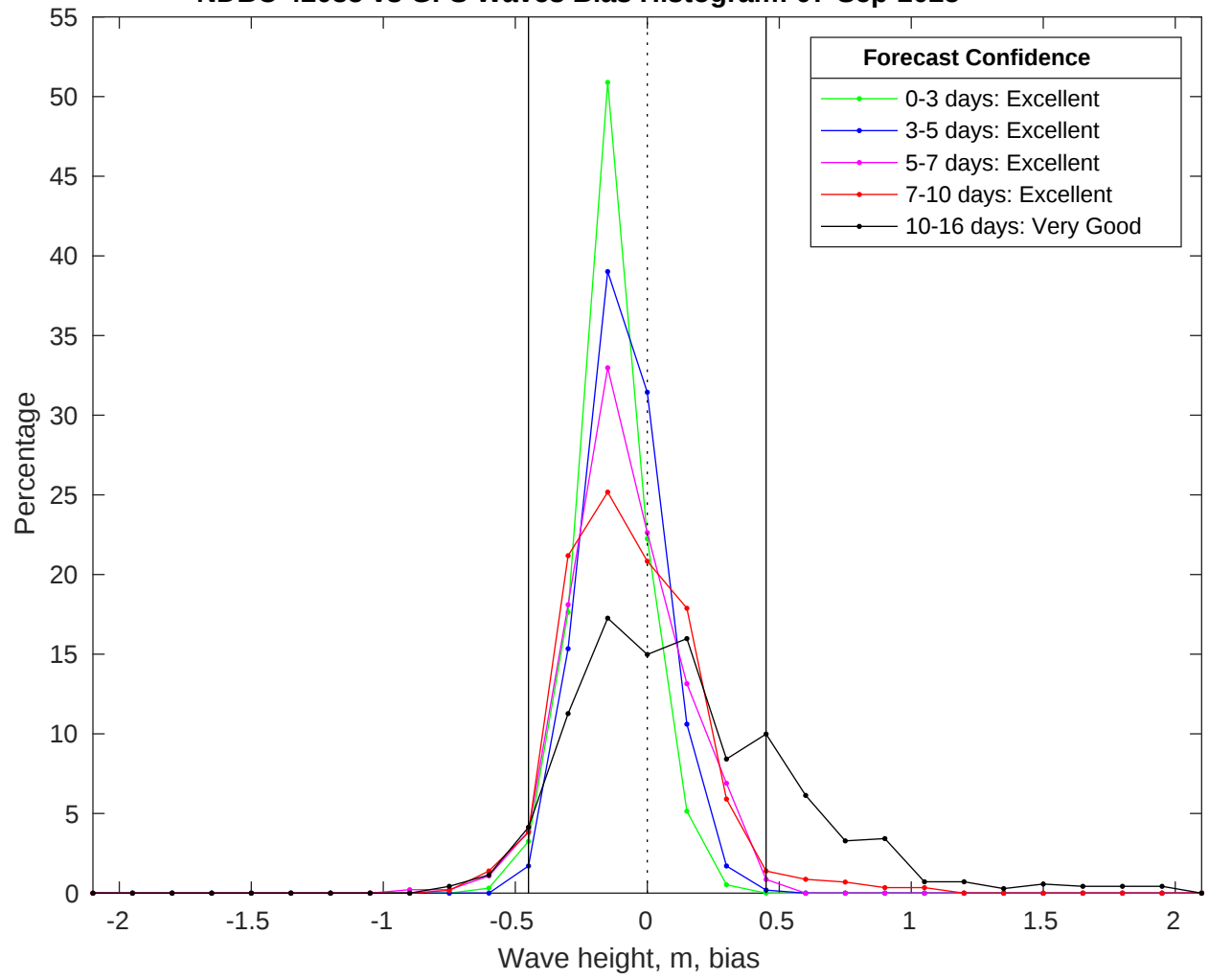
NDBC 42035 vs GFS Waves Bias Histogram: 07-Sep-2025
