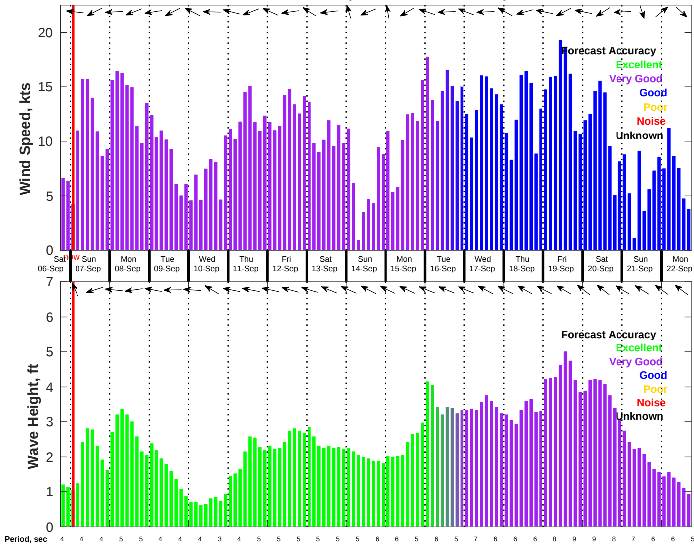
Wind & Wave Forecast for NDBC 42035 from 06-Sep-2025 18:00:00 to 22-Sep-2025 18:00:00
