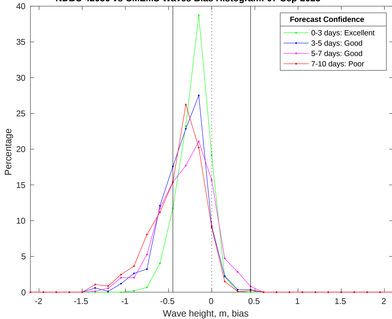
NDBC 42036 vs CMEMS Waves Bias Histogram: 07-Sep-2025
