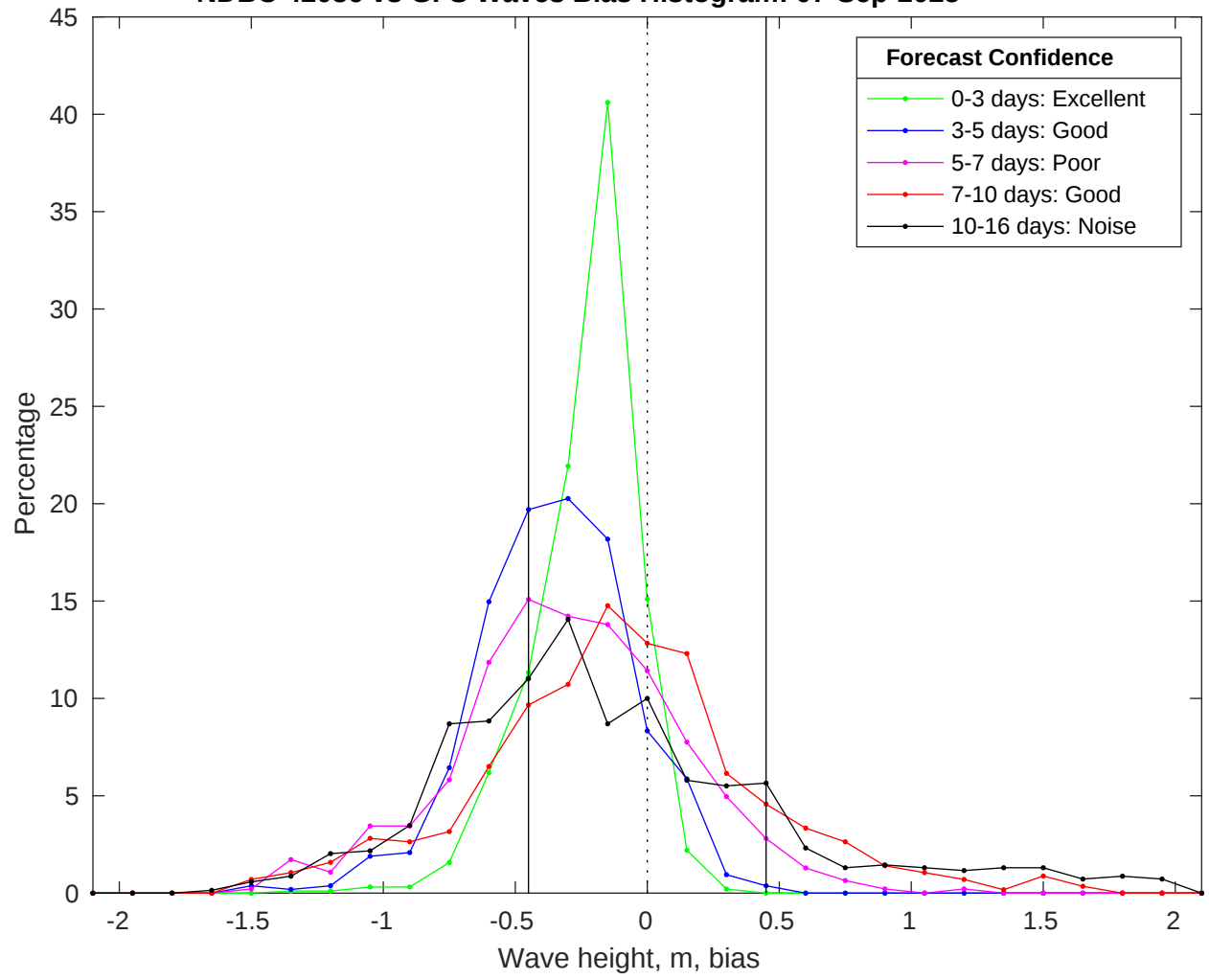
NDBC 42036 vs GFS Waves Bias Histogram: 07-Sep-2025
