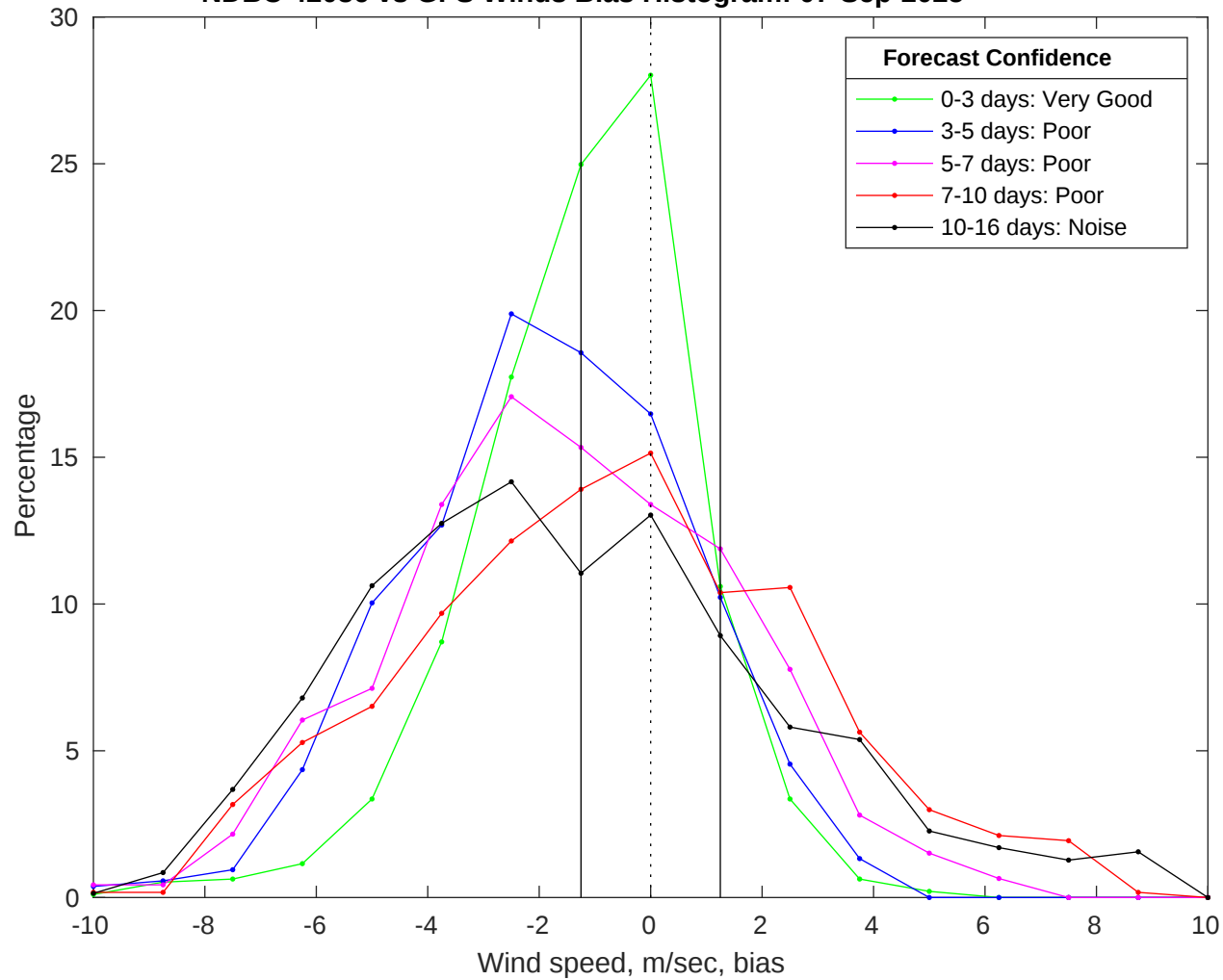
NDBC 42036 vs GFS Winds Bias Histogram: 07-Sep-2025
