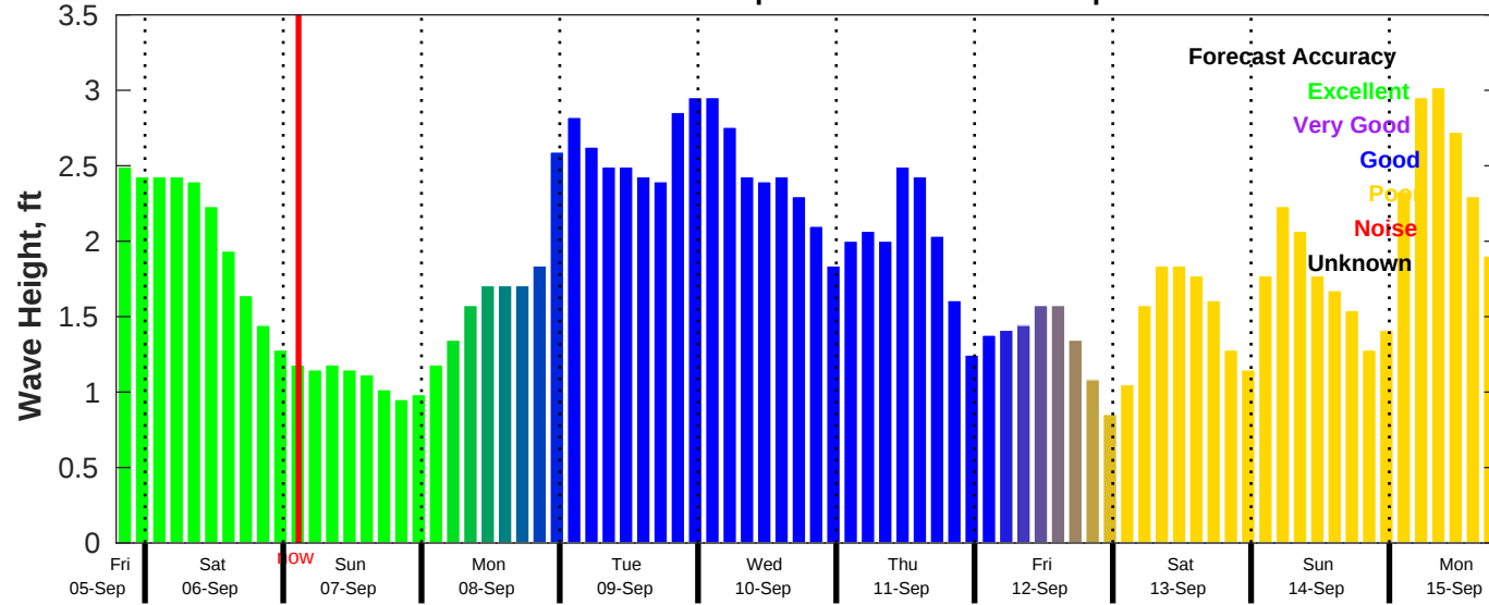
CMEMS Wave Forecast for NDBC 42036 from 05-Sep-2025 19:00:00 to 15-Sep-2025 19:00:00
